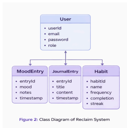
Figure 2: Class Diagram of Reclaim System
