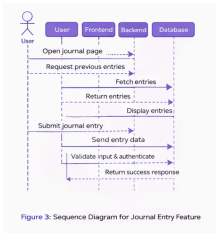
Figure 3: Sequence Diagram for Journal Entry Feature
